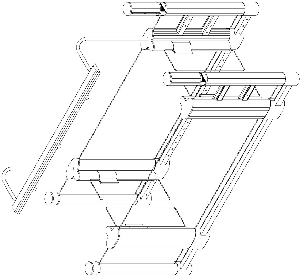
Perspective view
